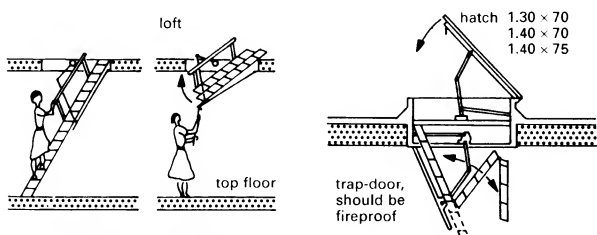
⑦ Space-saving, telescopic aluminium or wooden ladders for lofts → ⑤ + ⑥
